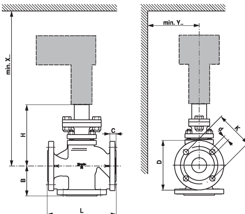
Dimensional drawings
